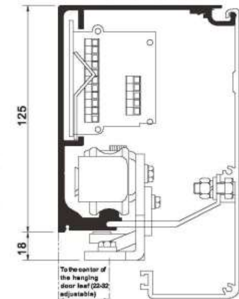
Sectional view
