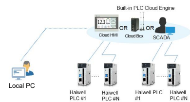
Local Programming
